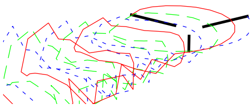
Calculated Forward Flight Free Wake Geometry
