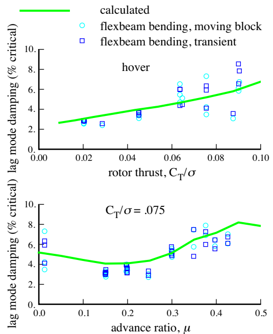
Bearingless Rotor Stability
